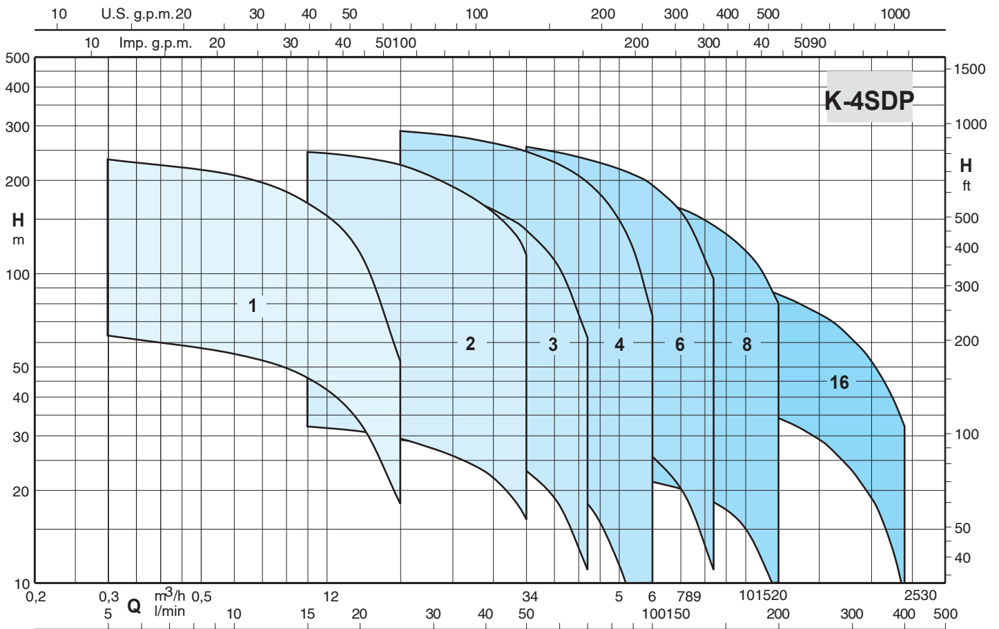
Coverage chart n \approx 2900 rpm
